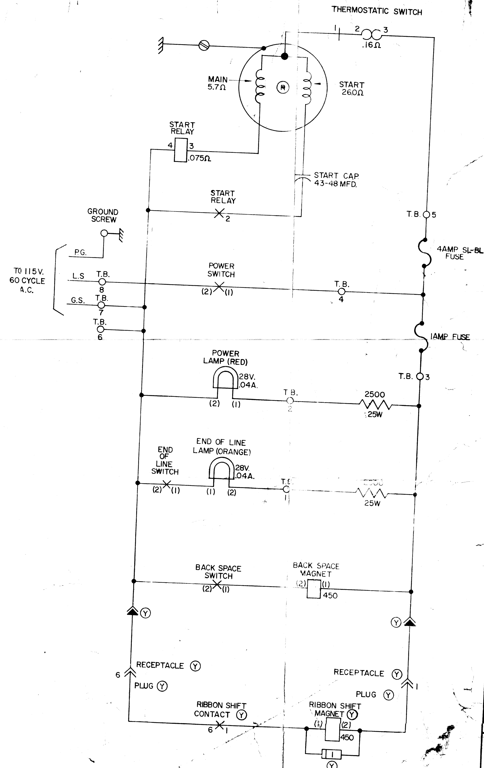
SCHEMATIC
